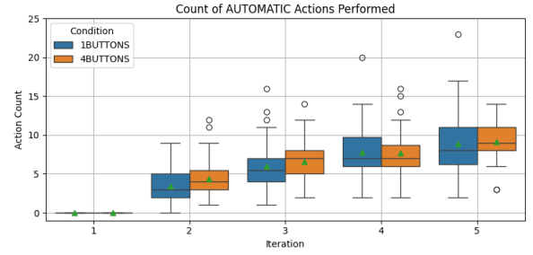
Fig. 3. Number of Automatic Actions Performed for Each Condition in Each Iteration
